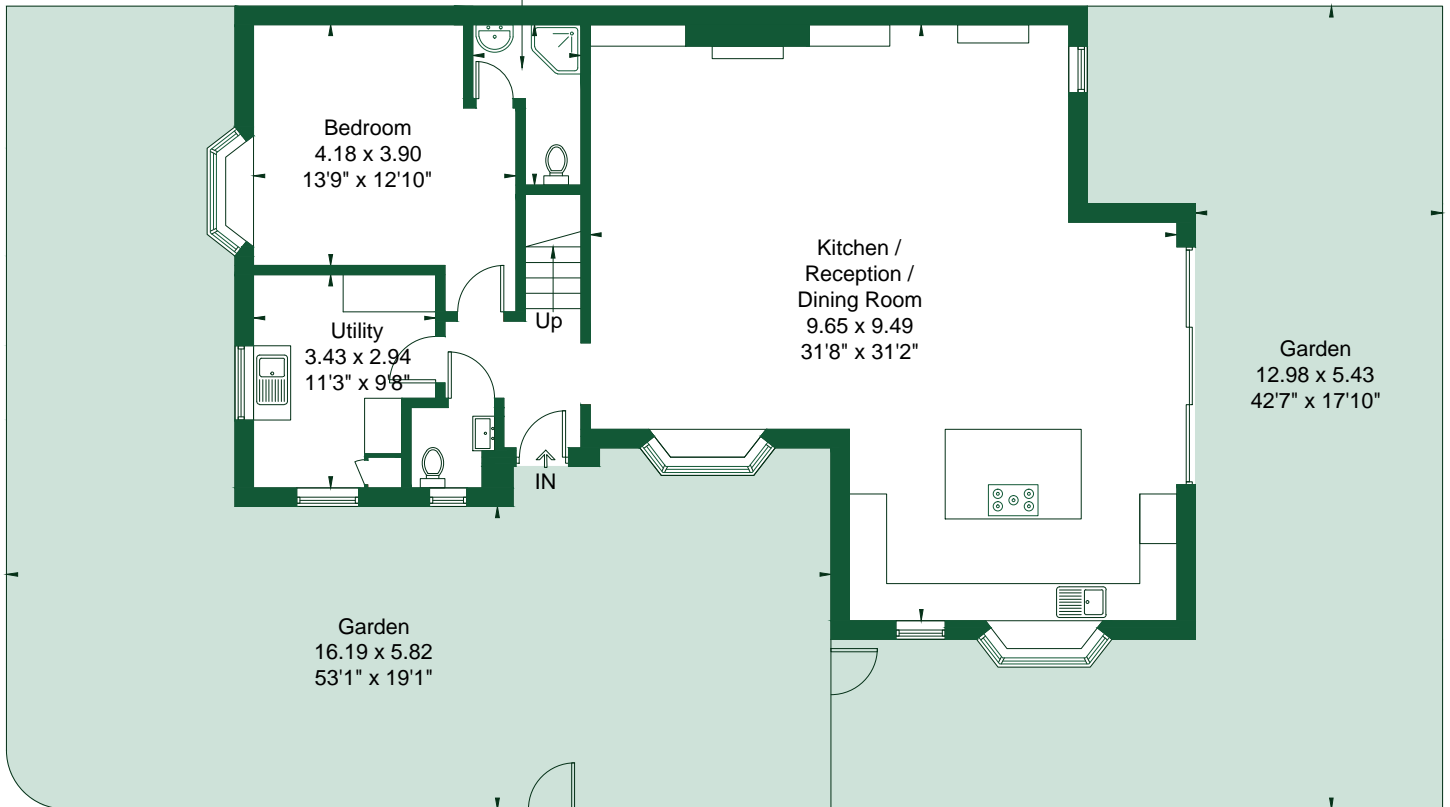
Ground Floor 114.9 sq m / 1236 sq ft
